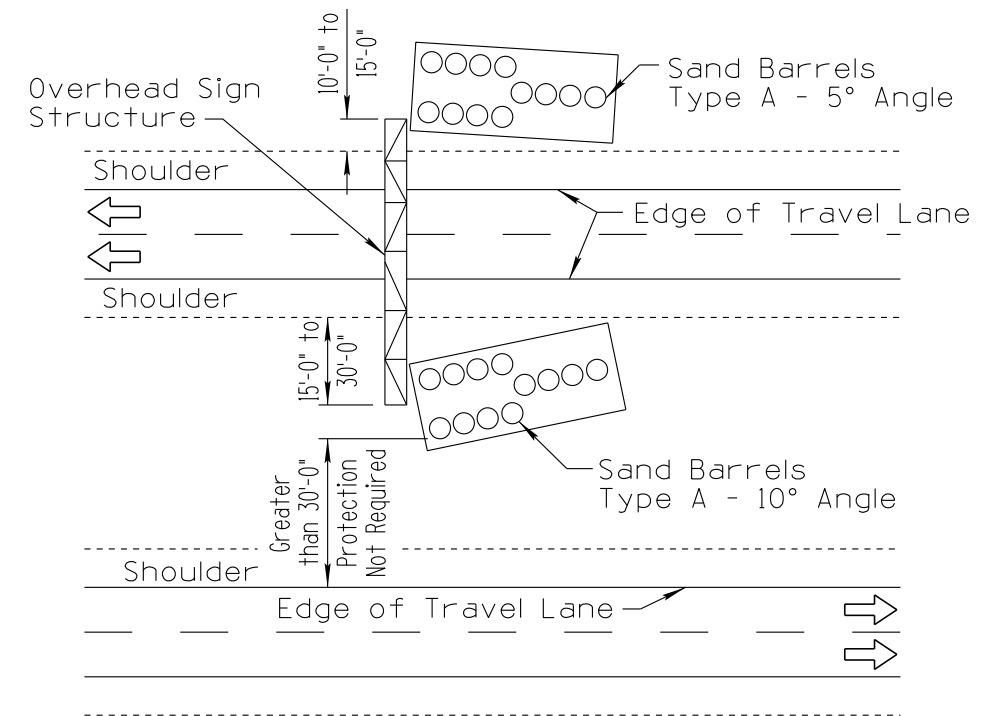
OVERHEAD SIGN STRUCTURE
