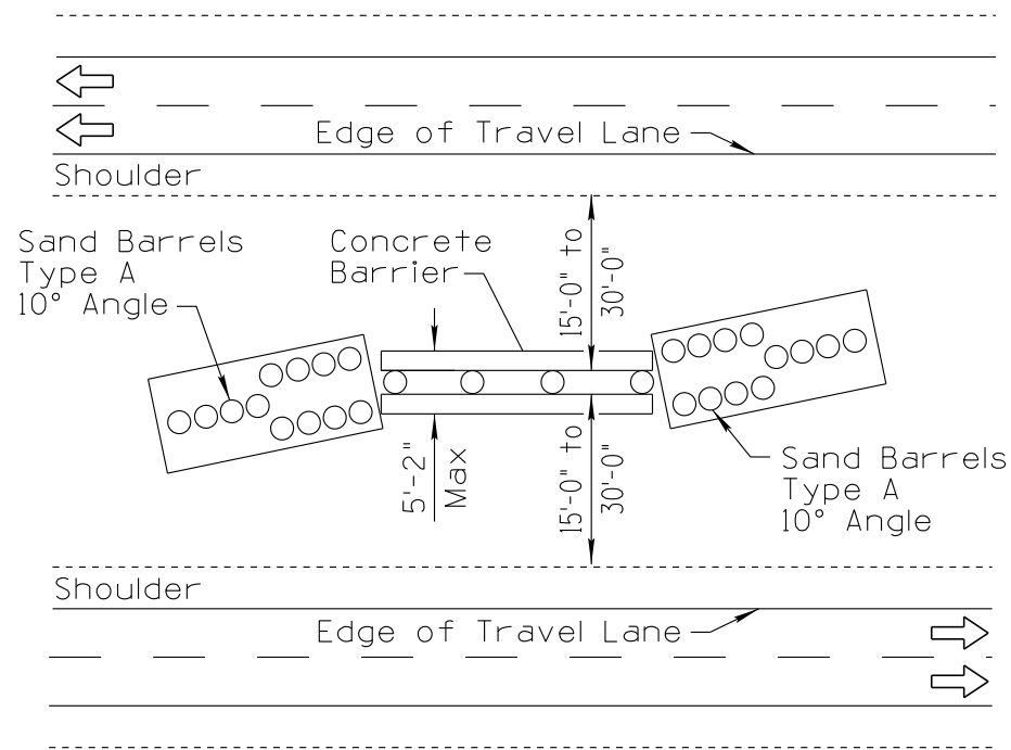
SINGLE PIER OR COLUMN
