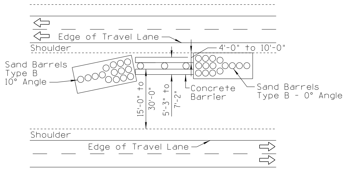
OFFSET SINGLE PIER OR COLUMN
