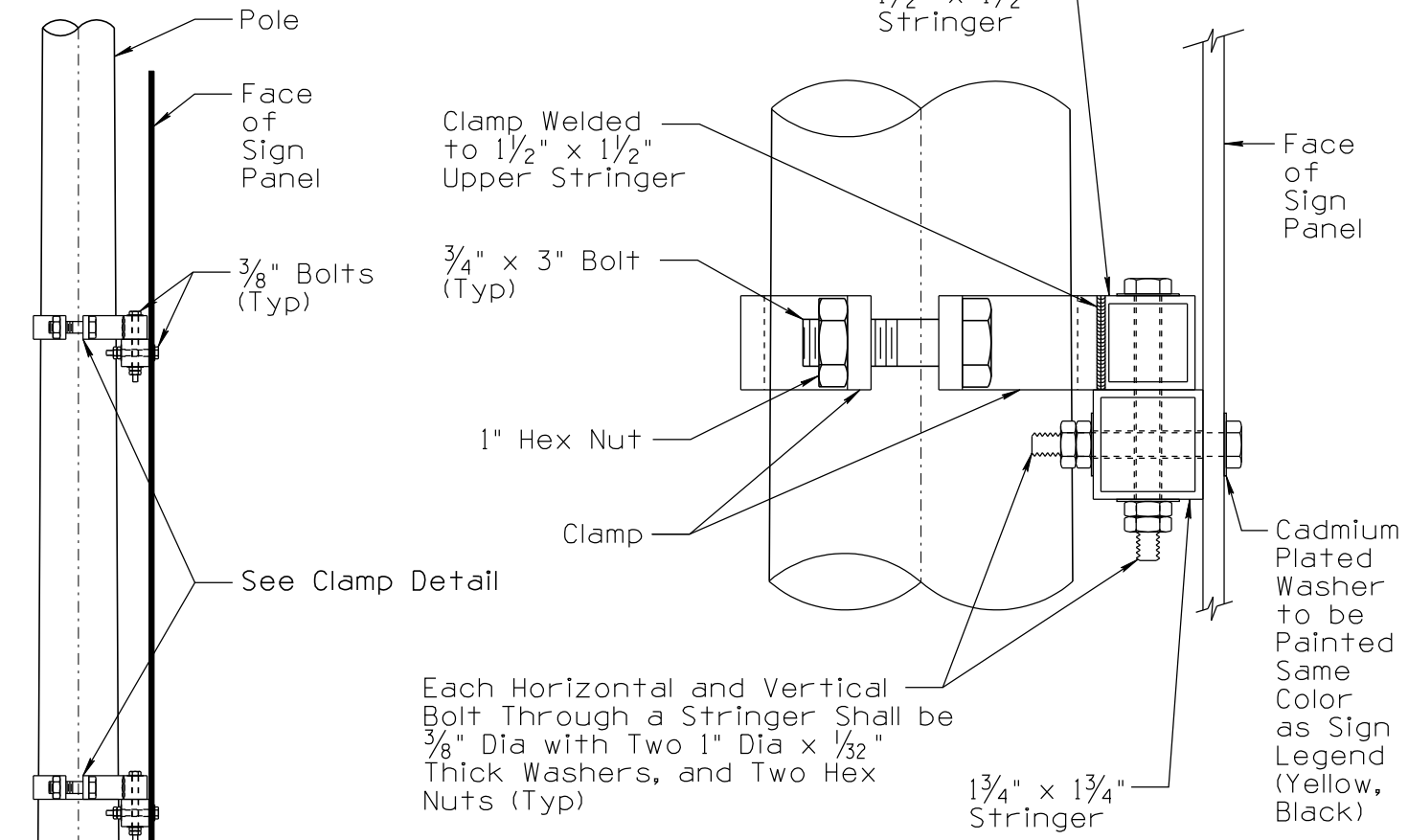
CLAMP DETAIL
