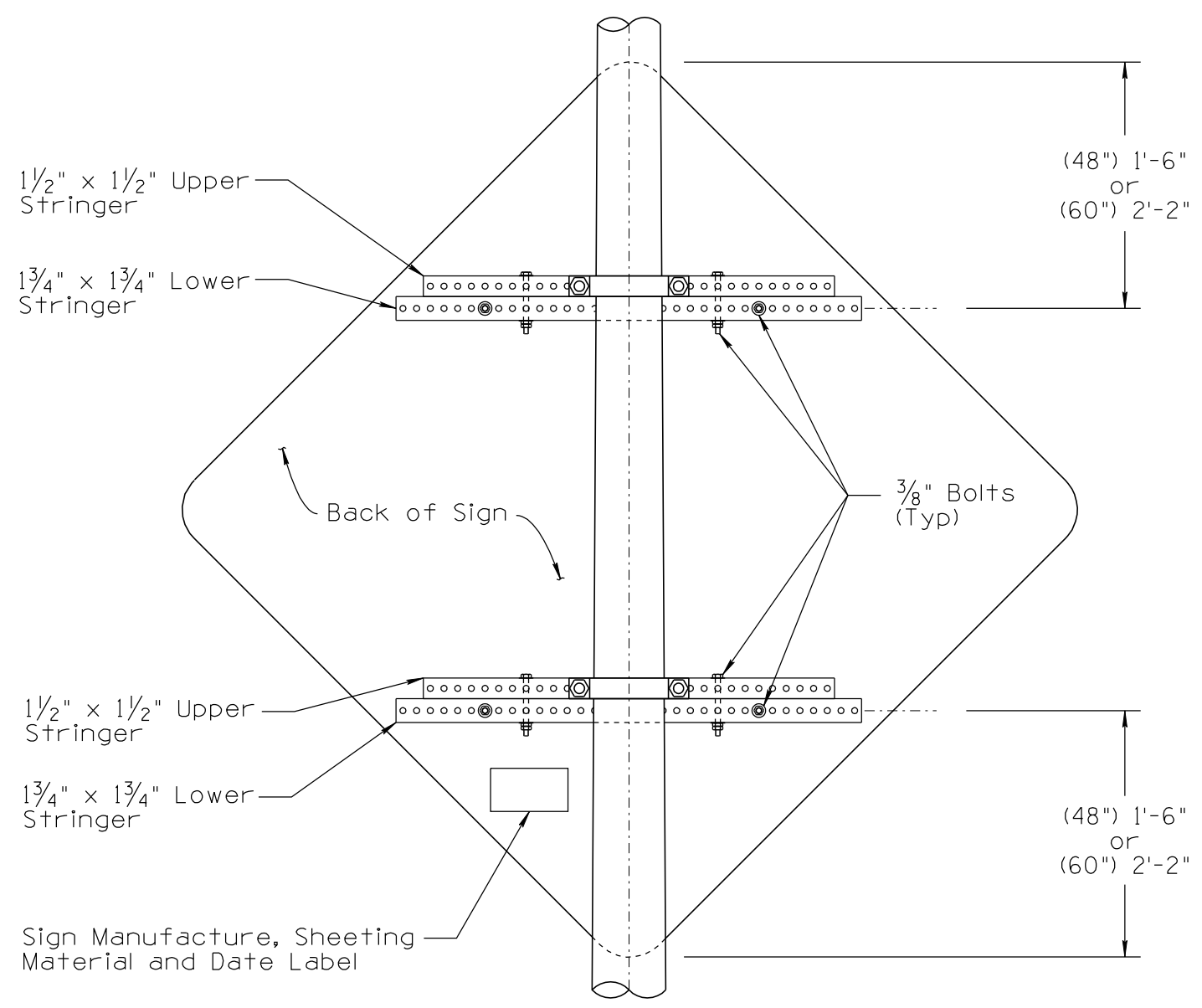
REAR VIEW (48" Sign Shown)
