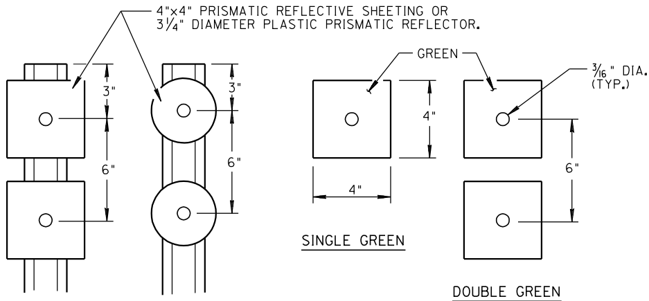
SNOW MARKER DETAILS
