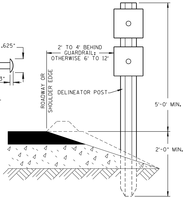
INSTALLATION DETAIL
