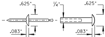
BLIND RIVET DETAIL
