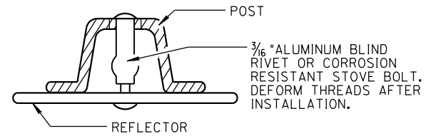
REFLECTOR ATTACHMENTS
