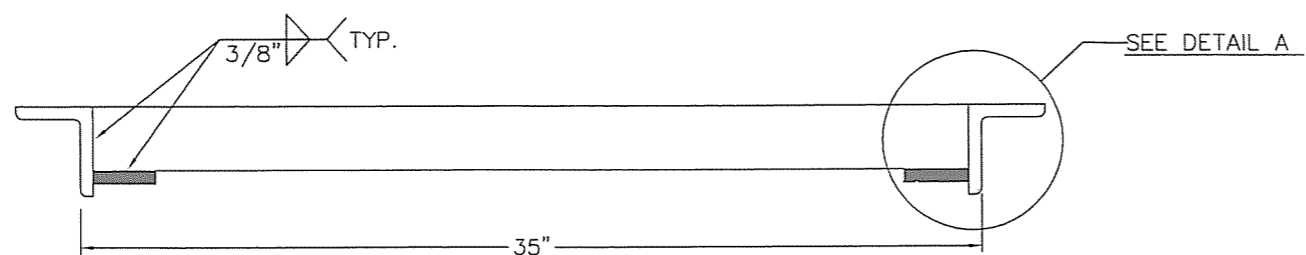
GRATE SIDE VIEW
