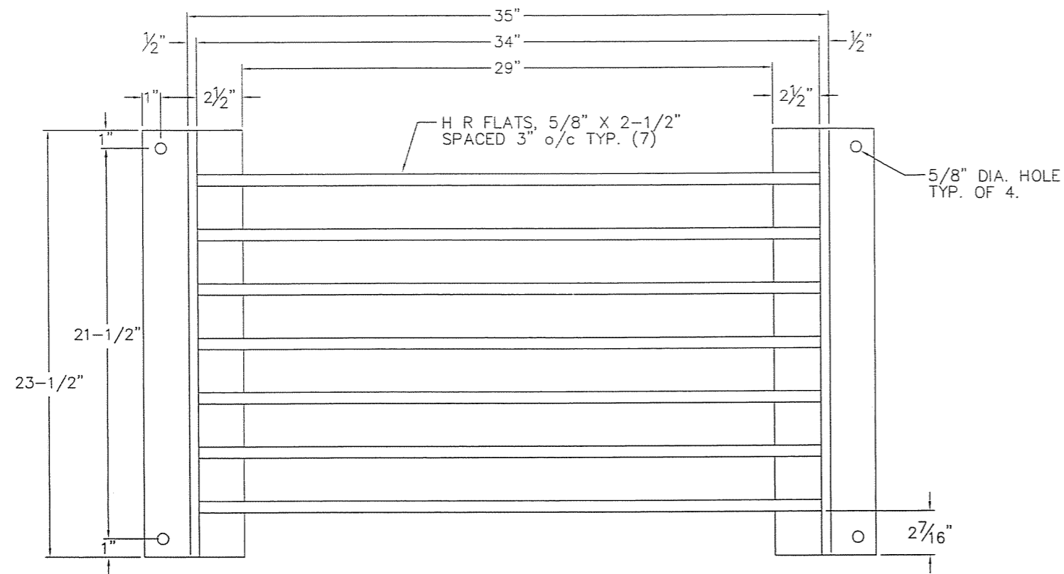
GRATE PLAN VIEW
