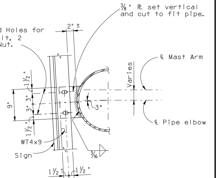
ELEVATION SIGN MOUNTING BRACKET AT ELBOW
