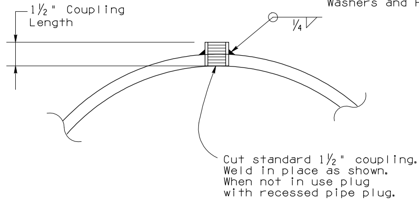
DETAIL D
