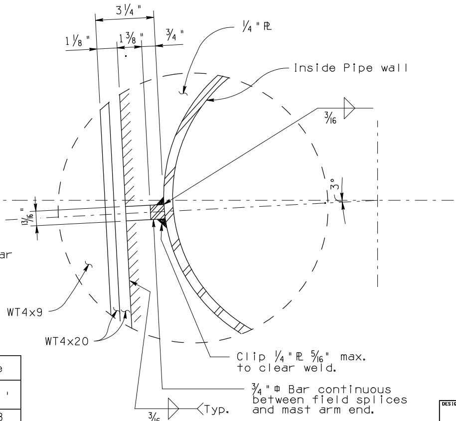
DETAIL E
