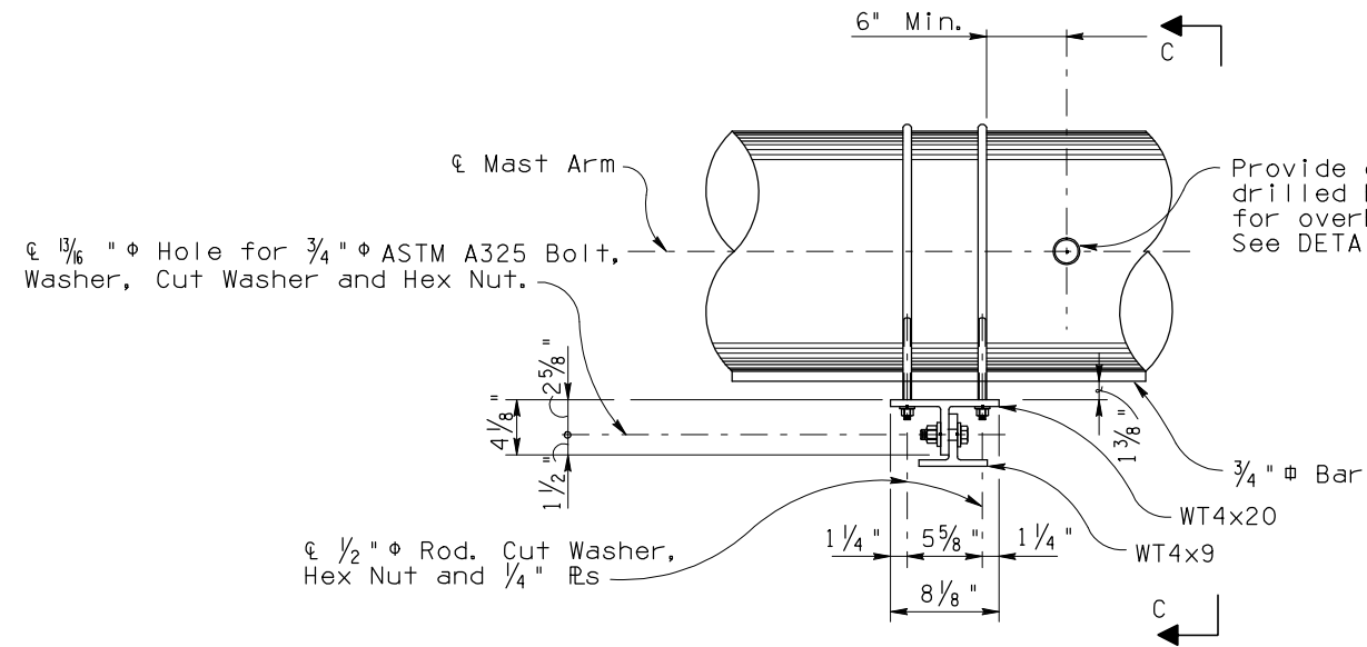
PLAN SIGN MOUNTING BRACKET
