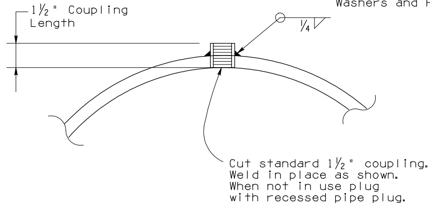
DETAIL D
