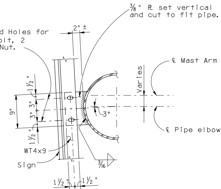
ELEVATION SIGN MOUNTING BRACKET AT ELBOW
