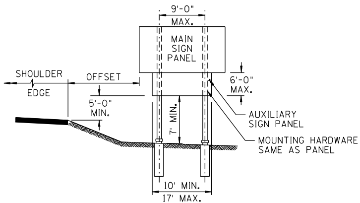
TWO POSTS SIGN POST SPACING LESS THAN WIDTH OF AUXILIARY SIGNS MINUS 1'-0"
