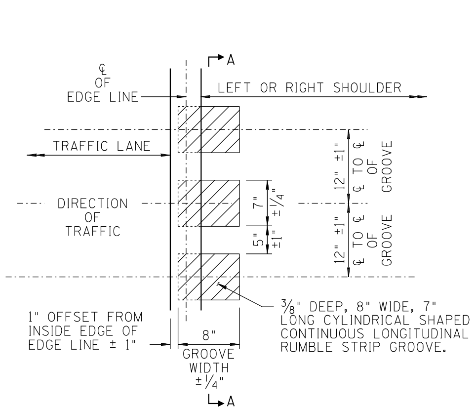
PLAN VIEW
